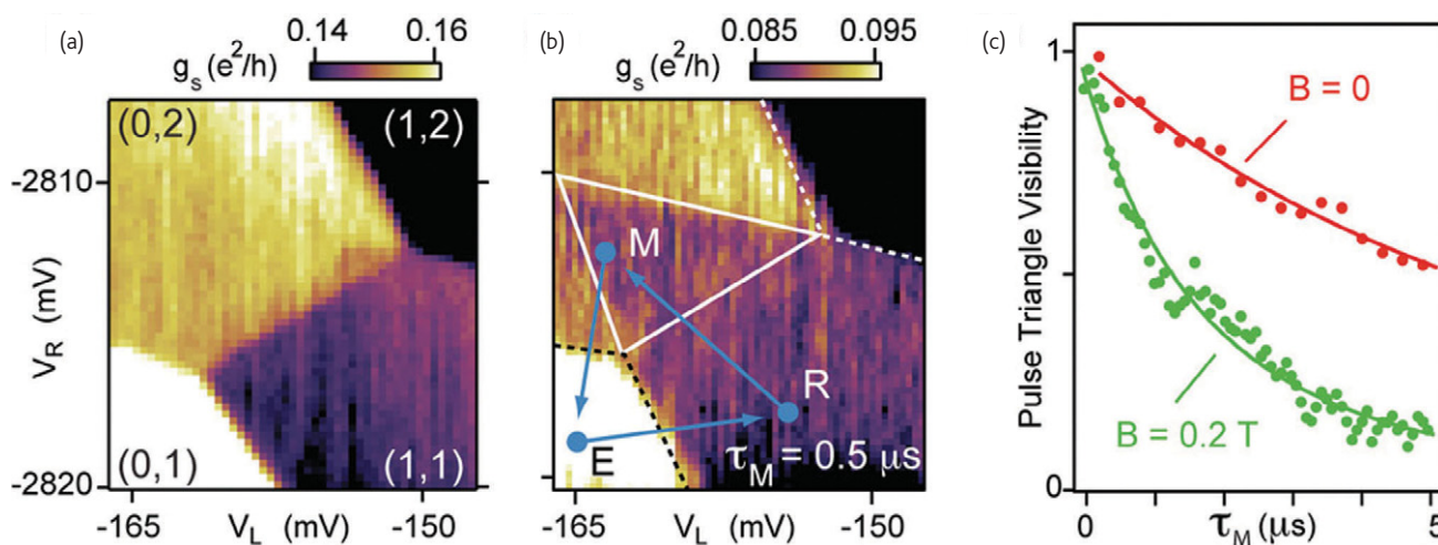
Fig. 9 Pulsed-gate measurements of spin-relaxation using charge sensing. (a) The conductance of the charge sensor g_s is a measure for the charge occupancy of the double quantum dot. (b) If the gate voltages are cycled between E, R and M faster than the spin-relaxation time, two separated electrons (1,1) may be prevented by their spin symmetry from tunneling into one dot (0,2). This results in a pulse triangle (white line) whose color sensitively depends on how much time \tau_M is spent at point M. (c) The relaxation time is extracted from the dependence of the pulse triangle color on \tau_M at various magnetic fields. (Parts (a, b) reprinted with permission from 20 © 2005 by the American Physical Society.)
