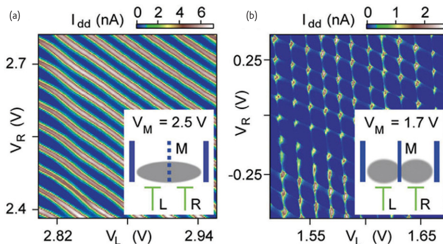
Fig. 7 Current I_{dd} through the carbon nanotube as a function of right and left gate voltages. (a) Coulomb oscillations indicate a single quantum dot that is capacitively coupled to both the left (L) and right (R) plunger gate. (b) Increasing the middle barrier (M) transforms the quantum dot into a double quantum dot, and the conductance is suppressed except near triple points 19 .
