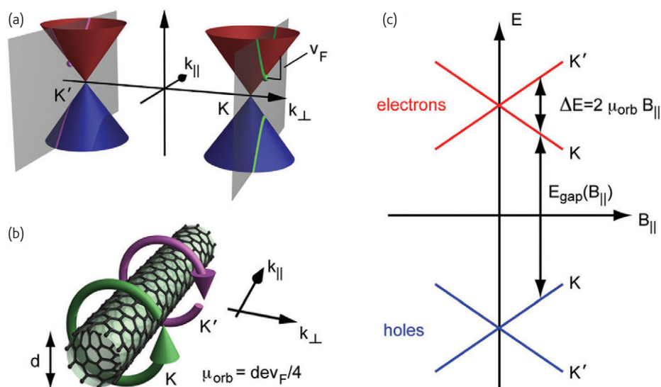
Fig. 2 Orbital electronic structure of NTs. (a) The quantization condition (gray planes) around the nanotube circumference results in four hyperbolic bands (green and purple) near the two Dirac points (K, K') of graphene. (b) The lowest electron-like states in the K and K' valley are equal in energy (green and purple dots in panel a), and constitute a clockwise and counterclockwise persistent ring current. (c) The resulting large orbital magnetic moments \mu_{\text{orb}} can be employed to lift the valley degeneracy or tune the bandgap E_{\text{gap}} with an external magnetic field B_{\parallel} .
