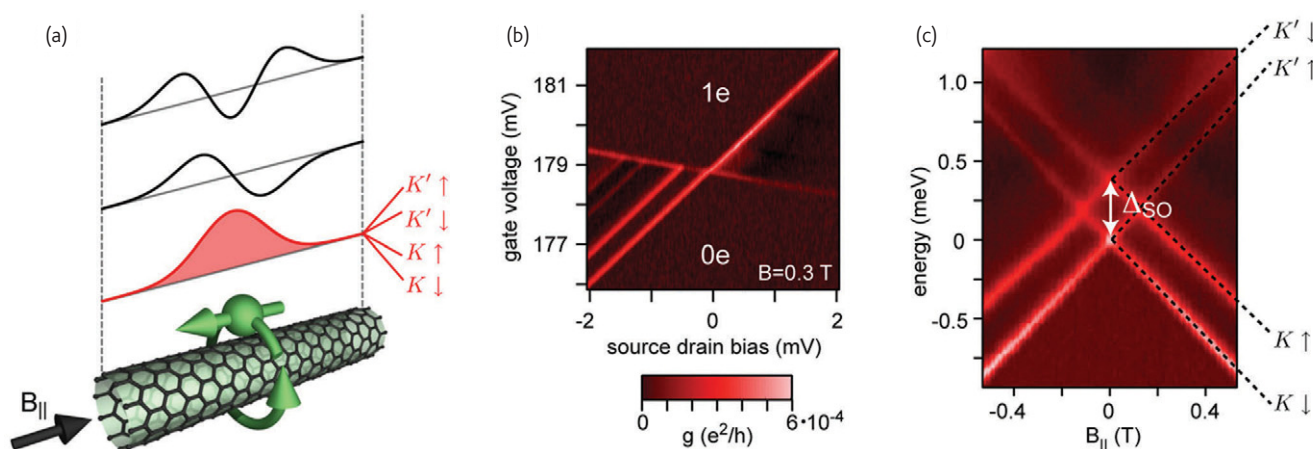
Fig. 4 (a) Understanding the four quantum states of the lowest electronic shell (red). (b) At sub-Kelvin temperatures and finite magnetic field the four combinations of clockwise/counterclockwise motion ( K/K' ) and spin up/down ( \uparrow/\downarrow ) are clearly resolved in a suspended device using tunneling spectroscopy. (c) Their magnetic field dependence reveals a spin-orbit gap of \Delta_{\text{SO}}=0.37 meV at zero magnetic field 18 .
