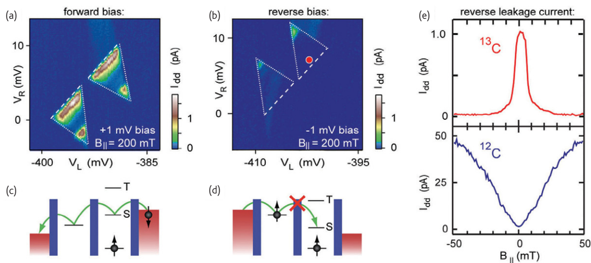
Fig. 8 Spin-blockade in a ^{13}\text{C} double quantum dot. (a) For positive bias current flow is observed near the base of the bias triangles (dashed line). (b) For negative bias current flow is strongly suppressed at finite magnetic field, indicating that spin selection rules prohibit interdot tunneling as schematically indicated in (d). (e) At zero magnetic field a small leakage current appears (top trace, measured near the red dot in panel b), indicating that electronic spins are efficiently flipped by nuclear spins. In contrast ^{12}\text{C} double quantum dots (lower trace) manifest a different behavior 19 .
