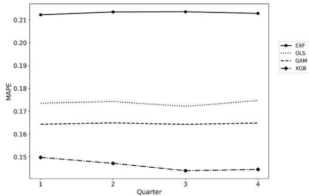
Fig. 3 Quaterly model error performance based on MAPE
