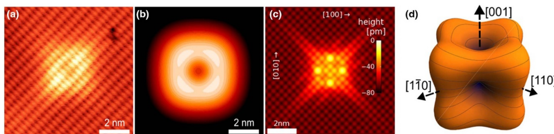
Figure 33. Subsurface acceptor states in silicon. (a) STM image a single acceptor located beneath the Si(001) surface, revealing characteristic spatial features of the bound hole state superimposed on the surface atomic lattice. (b), (d) Effective mass approximation calculations of an acceptor wave function in silicon; (b) shows the charge density evaluated for a plane 2.9 nm above the impurity layer along [001], while (d) shows a three-dimensional real-space iso-surface of the acceptor state wave function. (c) Tight-binding atomistic calculation of an acceptor wave function in silicon calculated for a depth of 0.81 nm. Reproduced from [296], with permission from ACS Publications.
