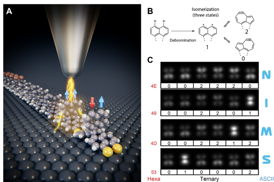
Figure 7. (A) Schematic drawing of memory bits using molecular networks under a tip of scanning tunnelling microscopy. (B) Example of three states isomerization. (C) Test recording with molecular bits in ternary cord. Reproduced from [83], with permission from Springer Nature.
