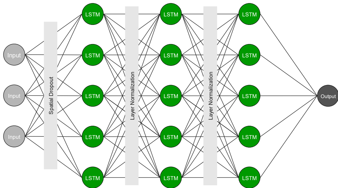
Figure 2.3 – LSTM Model
