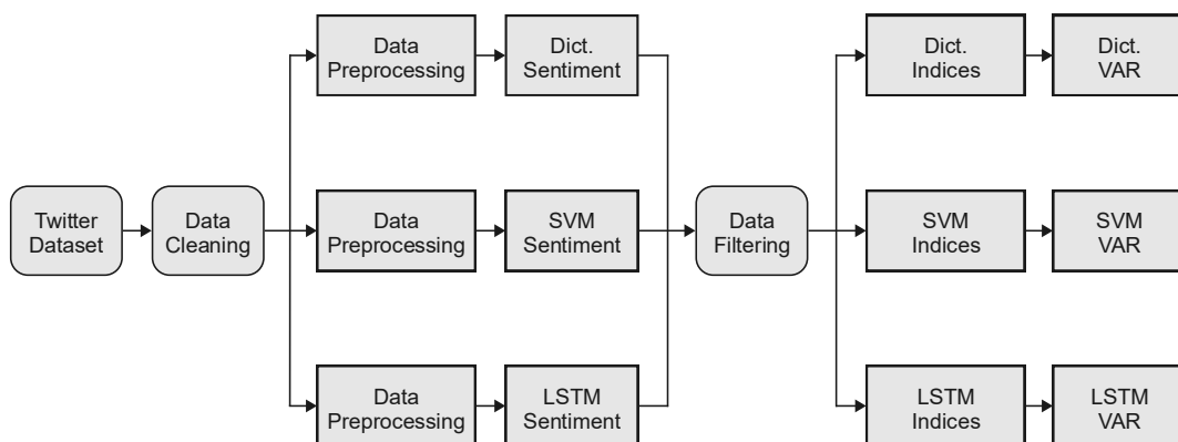
Figure 2.2 – NLP Process
