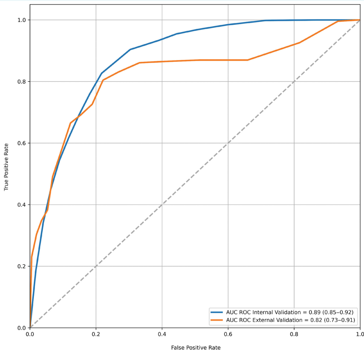
Figure 3 The receiver operating characteristic (ROC) curve. Mean ROC curves for the internal validation and external validation for 1000 bootstraps. The area under the ROC curve (AUC) is shown on the right corner. The dashed line (reference) represents a model with no skills.
