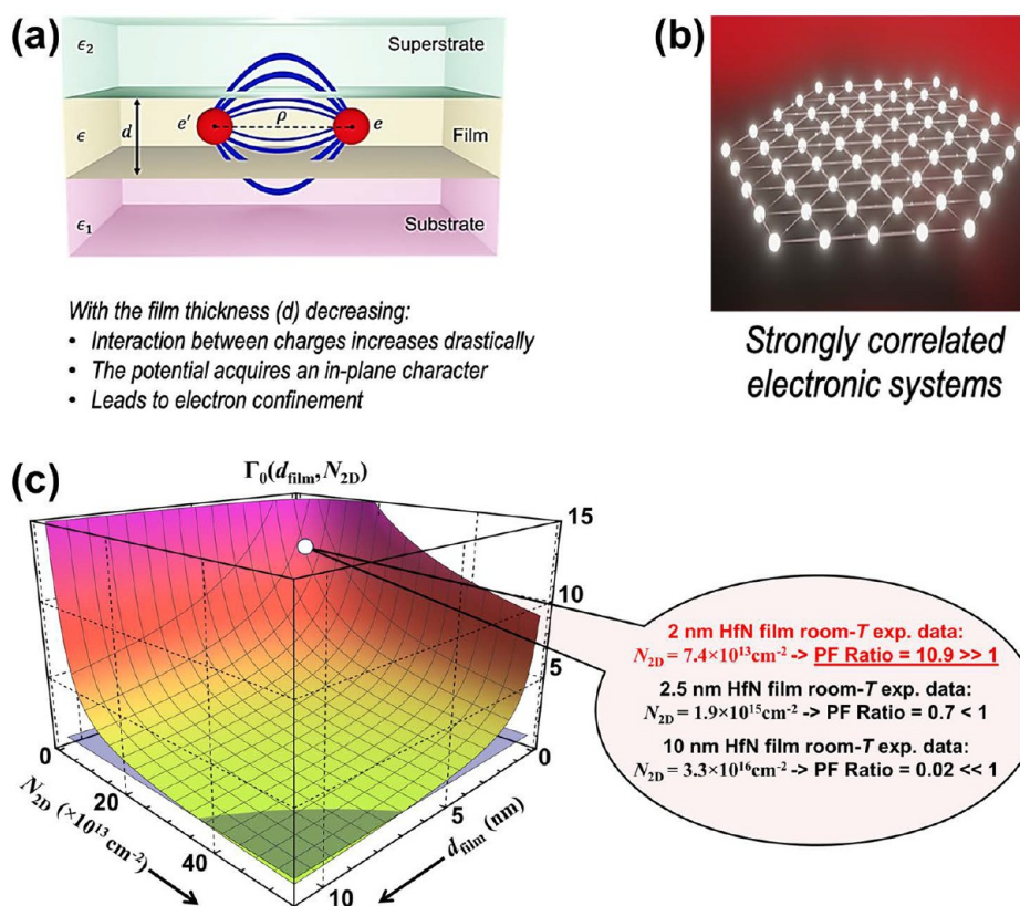
Figure 29. Strongly correlated electrons in transdimensional materials. (a) Electron confinement-induced plasmonic breakdown in a transdimensional material. We show a schematic of a plasmonic metal film sandwiched between a substrate and a superstrate. As the film thickness d decreases, the interaction potential among charges acquires an in-plane character and increases drastically, leading to electron confinement. (b) Schematic of Wigner crystallization when an interacting electron liquid has a sufficiently low electron density minimizing its total energy via crystallization into a quantum solid phase. 771 (c) Platzman–Fukuyama (PF) ratio given by eqs 29.1 and 29.2 plotted as a function of the surface charge density and film thickness with experimentally measured parameters of HfN TD films at room temperature. 800
