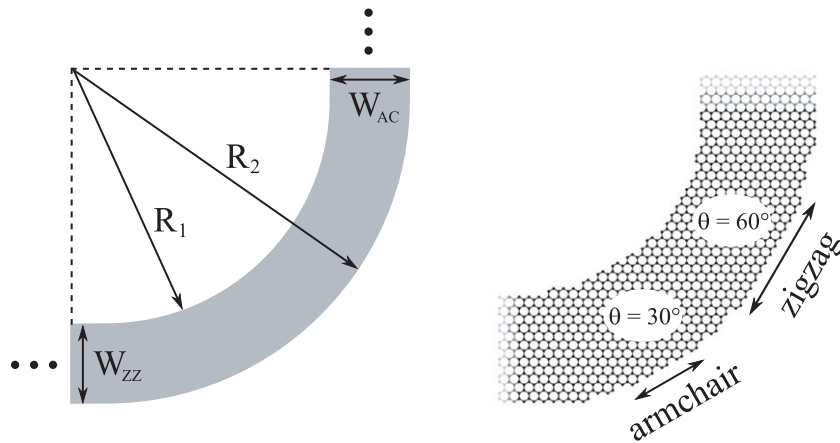
Figure 9. 90° curve with horizontal zigzag lead and vertical armchair lead. A local armchair region forms at \theta = 30^\circ and a local zigzag region at \theta = 60^\circ .
