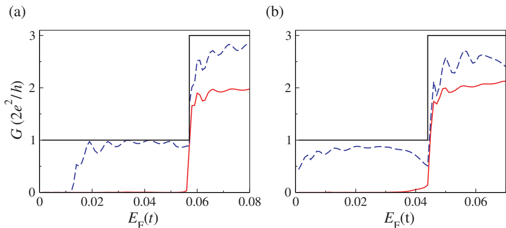
Figure 10. Conductance of 90° curved nanoribbons with either a semiconducting (solid red) or metallic (dashed blue) armchair region at \theta = 30^\circ . (a) Semiconducting armchair lead: W_{ac} = 69 (solid red) and W_{ac} = 69.5 (dashed blue). (b) Metallic armchair lead: W_{ac} = 88.5 (solid red) and W_{ac} = 89 (dashed blue). Black line: number of propagating modes in the zigzag lead ( R_2 = 259 ).
